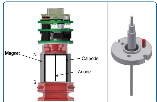
970 Series Inverted Magnetron (left); Anode Module (right)
