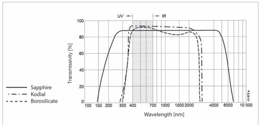
Optical transmissivity for the CF Sapphire observation windows
